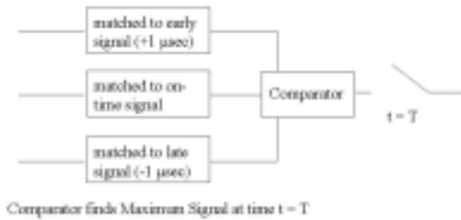
Figure 3. PPM Matched Filter
