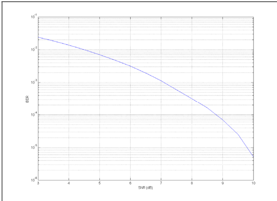
Figure B2: Uncoded bit error rate vs. received SNR for the proposed signal
