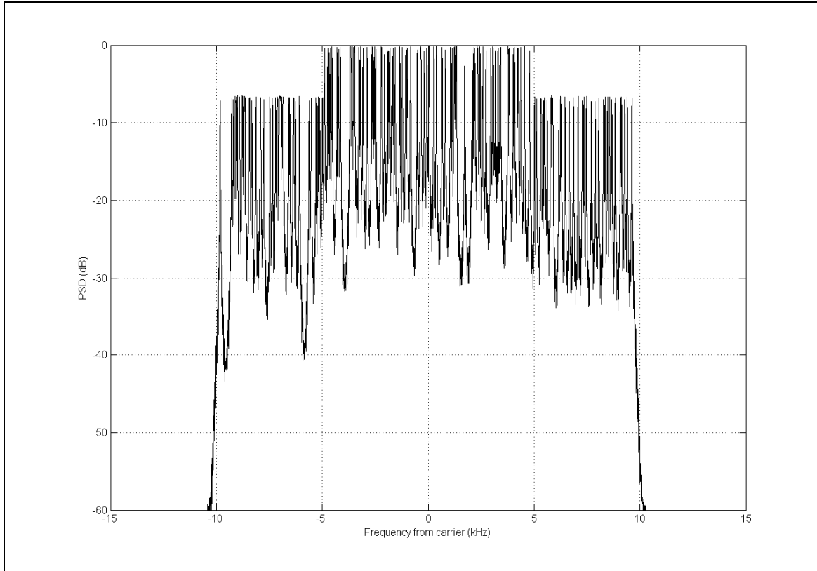
Figure B1: Power spectral density of the proposed signal using a 10 Hz resolution bandwidth
