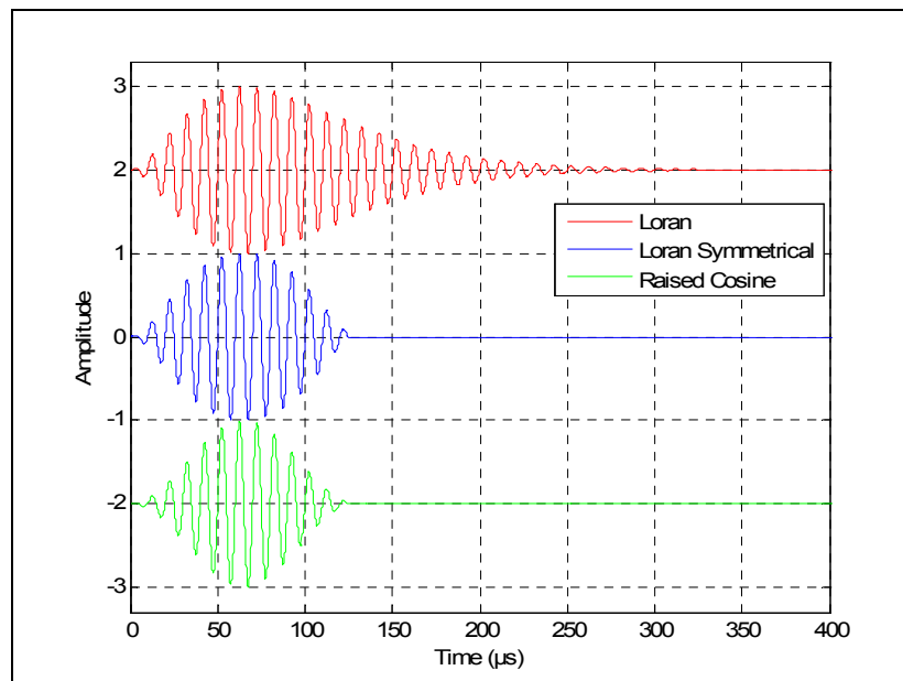
Figure C2: Time domain response
