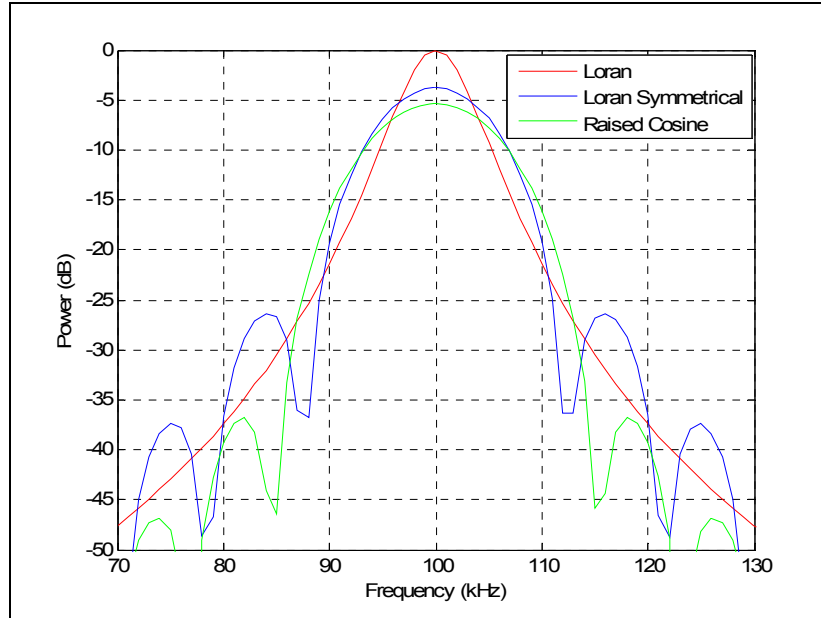
Figure C3: Frequency domain response
