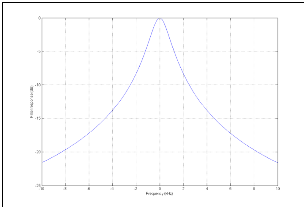
Figure B3: Frequency response of a transmitter filter and antenna with a combined Q of 60
