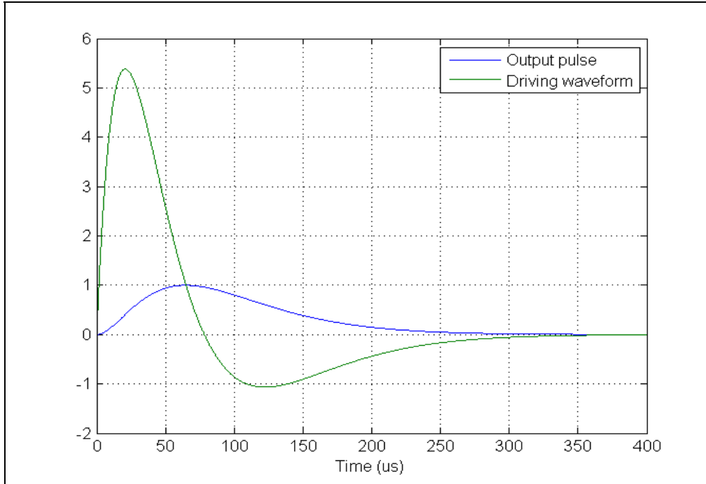
Figure B4: Desired Loran pulse along with the driving waveform required to achieve it into an antenna system with a Q of 60
