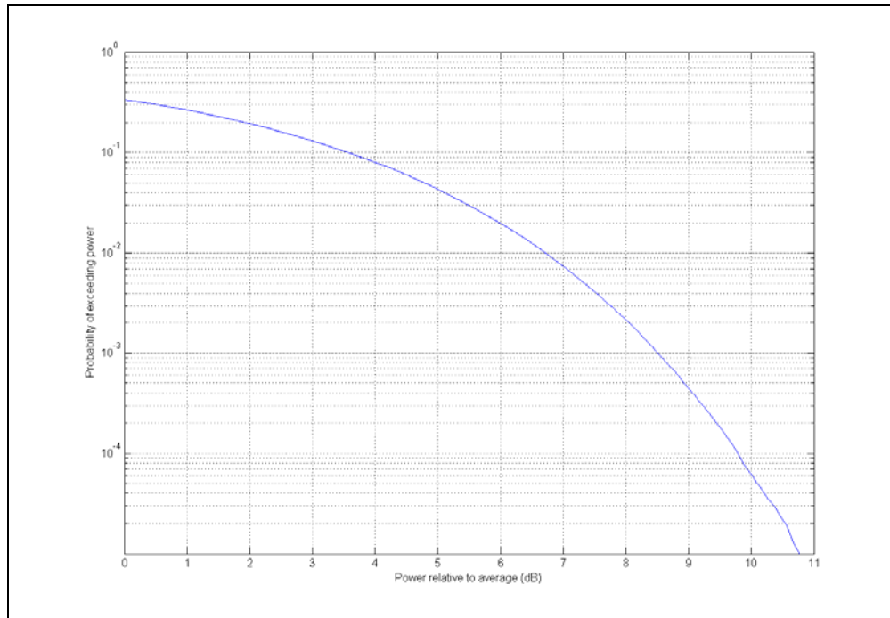
Figure B5: Signal CCDF, showing the probability of exceeding various power levels relative to the average
