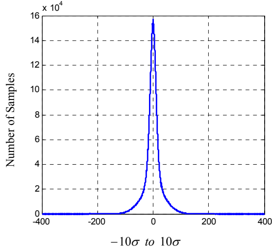
Figure 11. E-field antenna channel noise distribution for the first flight experiment
