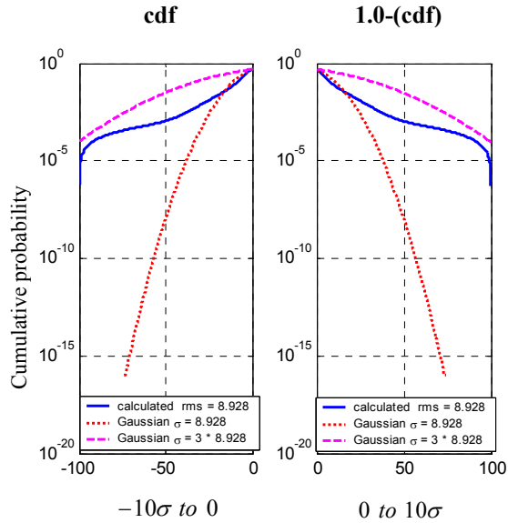
Figure 26. H-field antenna channel noise statistics for the second flight experiment
