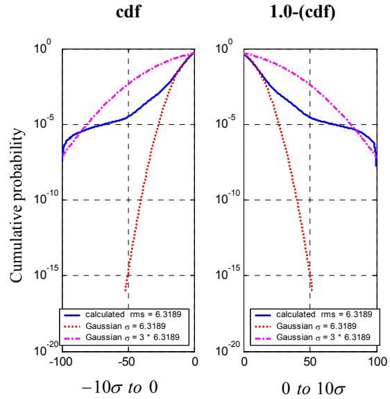
Figure 16. H-field antenna channel noise statistics for the first flight experiment
