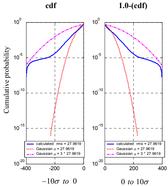
Figure 12. E-field antenna channel noise statistics for the first flight experiment
