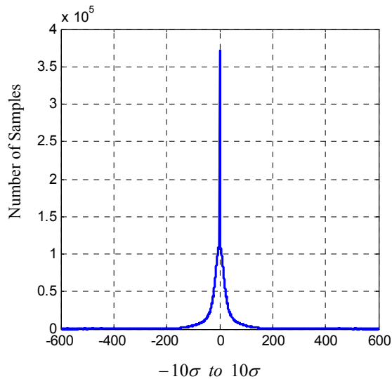
Figure 23. E-field antenna channel noise distribution for the second flight experiment
