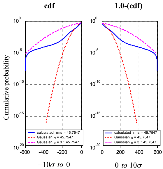
Figure 29. E-field antenna channel noise statistics for the third flight experiment
