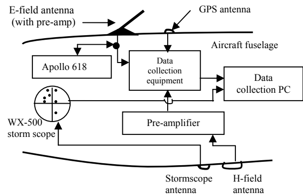
Figure 4. Flight Test Equipment Block Diagram
