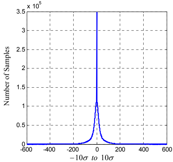
Figure 28. E-field antenna channel noise distribution for the third flight experiment
