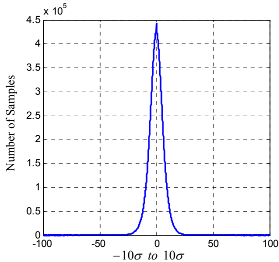
Figure 15. H-field antenna channel noise distribution for the first flight experiment
