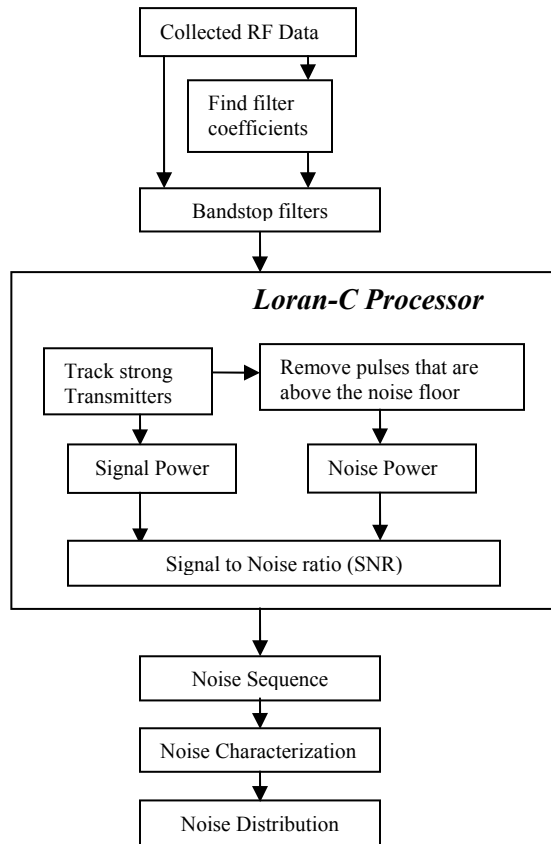
Figure 5. Data Processing Overview
