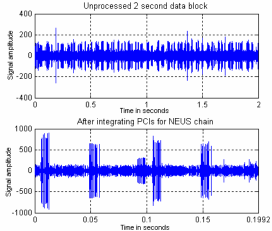
Figure 13. H-field antenna channel unprocessed 2-sec data block (top plot) and results after integrating over the PCI the NEUS chain (bottom plot) for the first flight experiment
