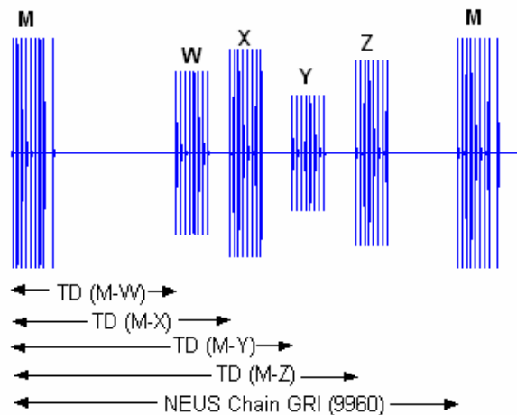
Figure 2. Received pulse pattern for the NEUS chain
