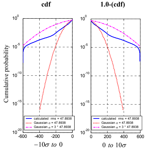
Figure 24. E-field antenna channel noise statistics for the second flight experiment
