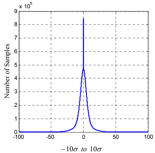
Figure 25. H-field antenna channel noise distribution for the second flight experiment
