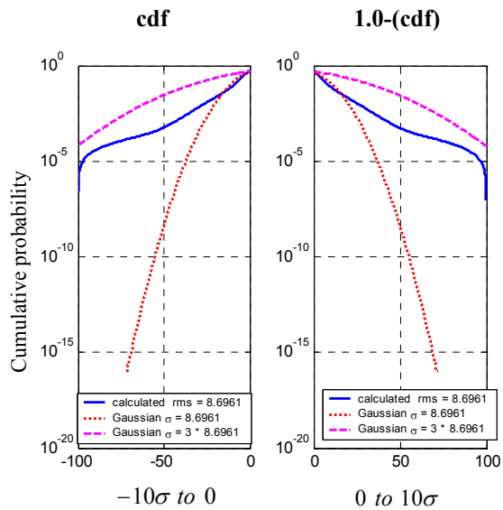
Figure 31. H-field antenna channel noise statistics for the third flight experiment
